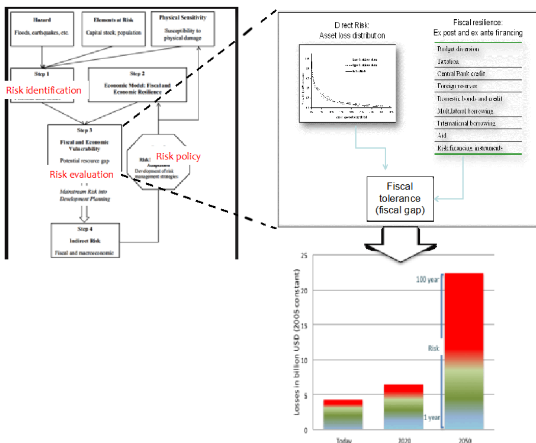
Figure 32: Assessing fiscal tolerance to extreme climate-related events: case of Bangladesh. Based on Mechler et al., 2014; Mechler and Bouwer, 2015
