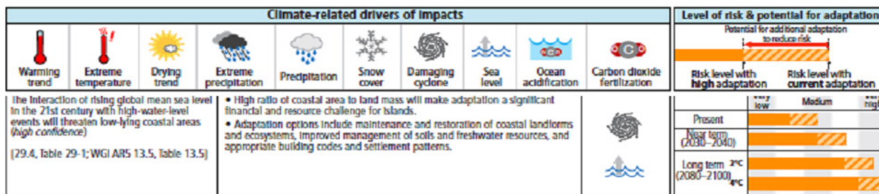
Figure 29: Risk from sea level rise & high-water events in Small Island States. Nurse et al., 2014
