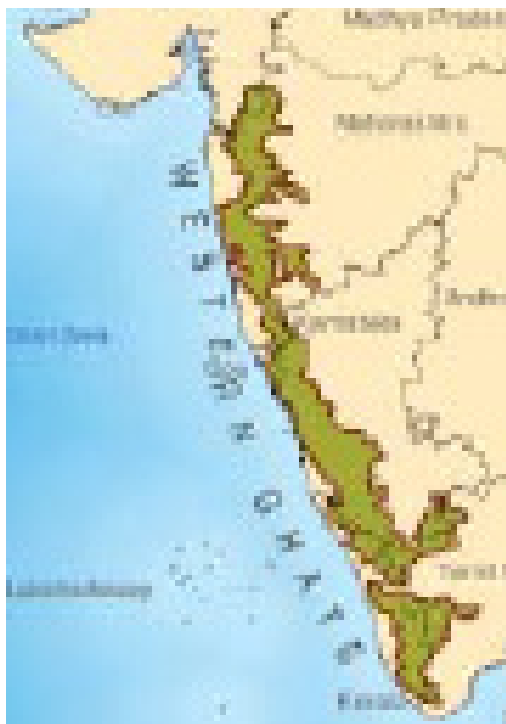
Figure 14: Western Ghats
